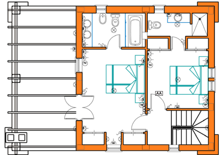
Planta Alta y Solarium / First Floor and Sun Terrace
