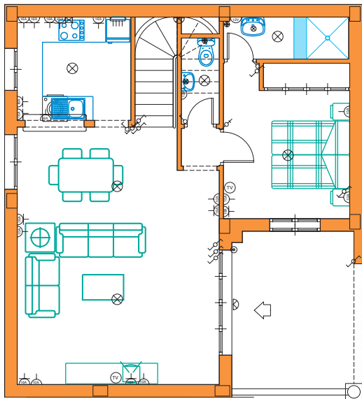
Planta baja Ground floor
